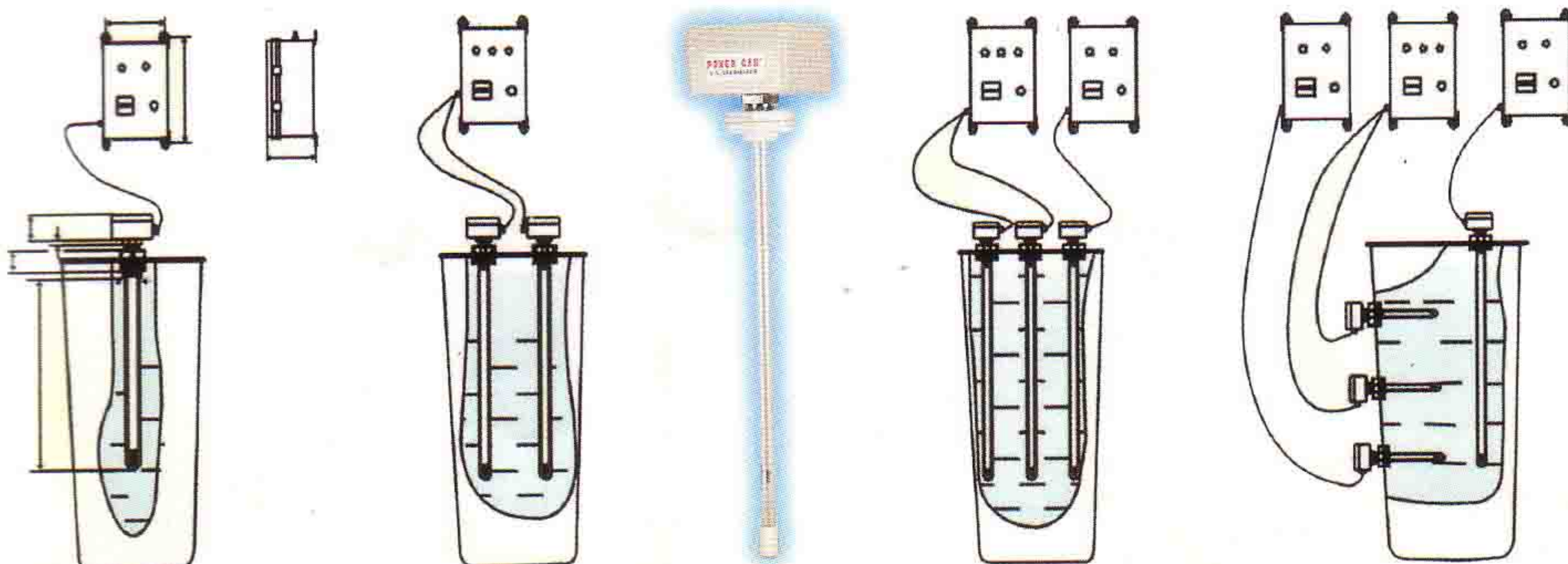
INSTALLATION DIAGRAM
