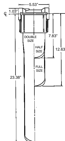
Housing without pressure relief button
